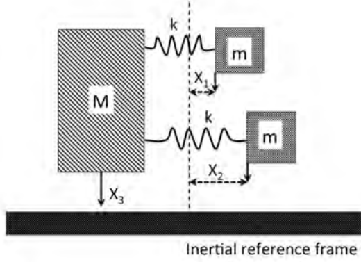
Fig. 1. The coupled oscillator system considered in our study.
