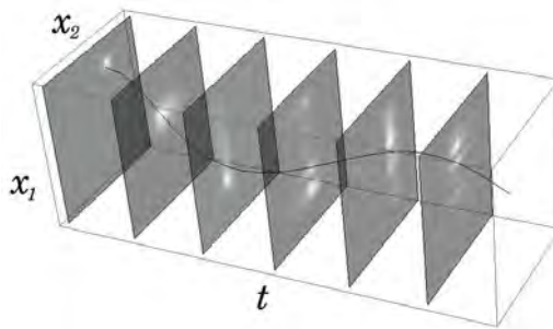
Fig. 3. Evolution of the system's wave function in the x_1, x_2 coordinate plane. The line is the trajectory of the expectation value of the system's coordinates.
