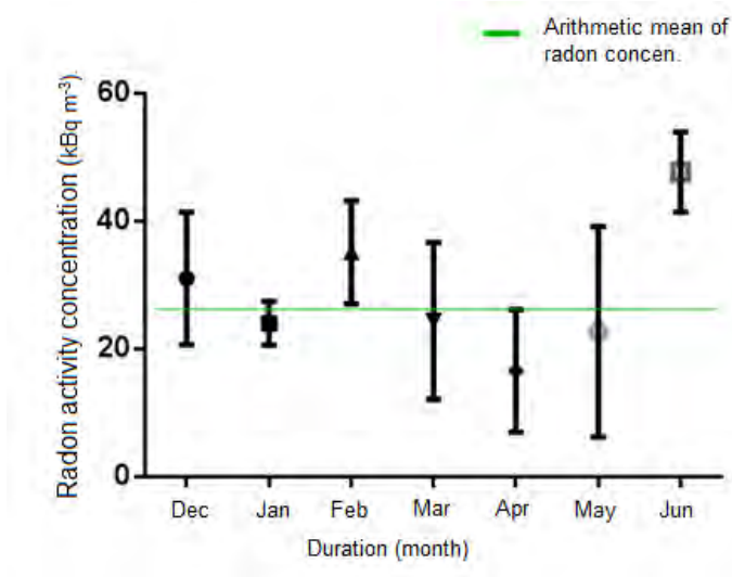
Fig. 5. Arithmetic mean of radon concentration with confidence interval of 95%
