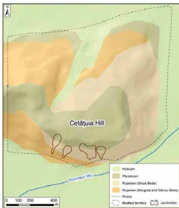
Fig. 2. Geological map
