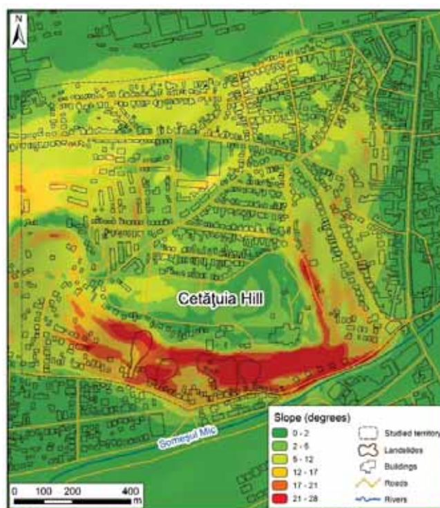
Fig. 4. Slopes map
