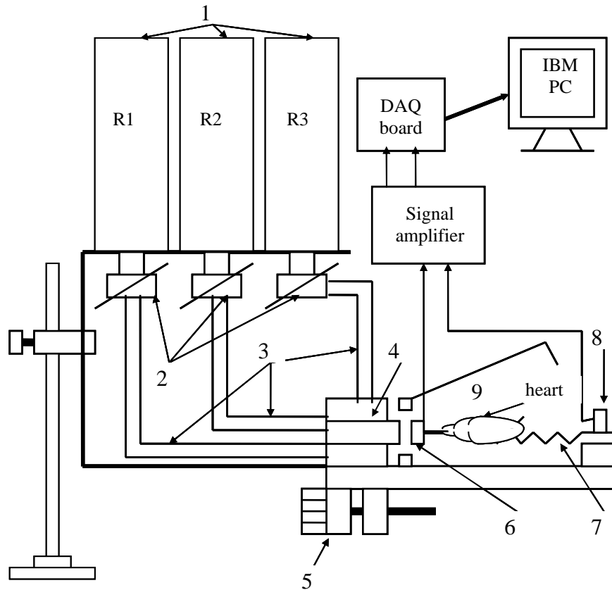
Fig. 1. Schematic diagram of the data acquisition system. 1 - Perfusing reservoirs. 2 – Taps. 3 - Plastic tubes. 4 - Perfusing head. 5 - Displacement device. 6 - Perfusion cannula/reference electrode. 7 - Active electrode. 8 – Pincers. 9 - Perfusion chamber.
